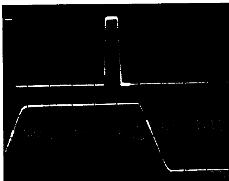
Figure 3. With the B sweep triggered, the width to be measured is within the intensified zone and polarity is selected by the B trigger slope control.
