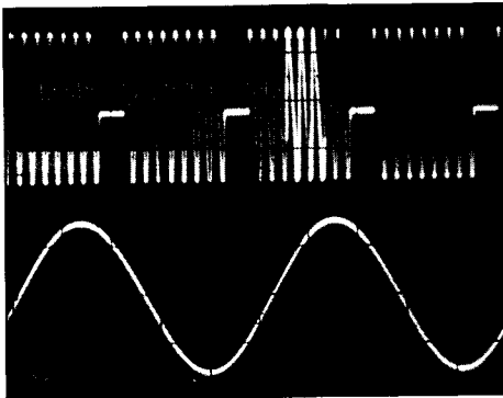
Figure 1. With the B sweep triggered, the frequency within the intensified zone on the A sweep is measured.
